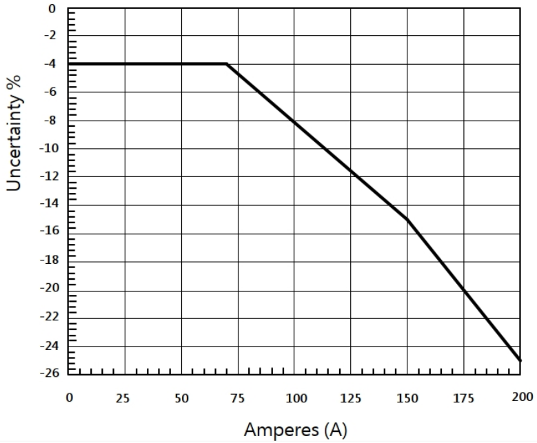
Figure 8: DC signal linearity in the 10 mV/A range, typical
