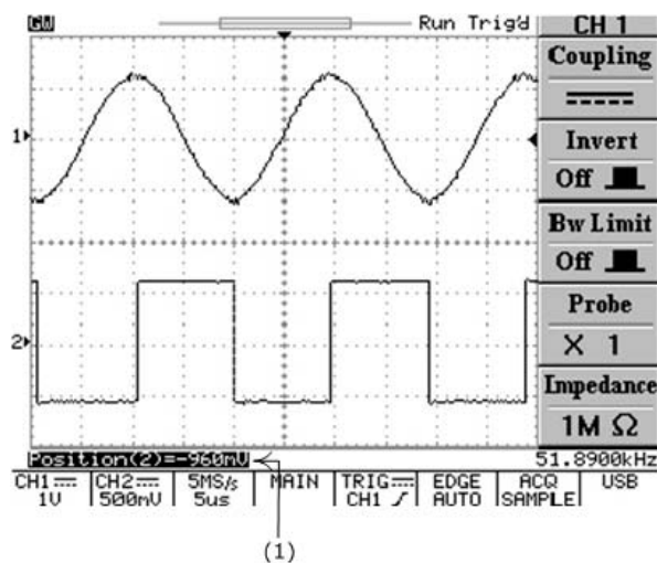
Figure 5-2: Operating the position knob
