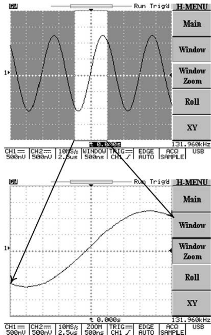
Figure 5-6: Operating the zoom function
