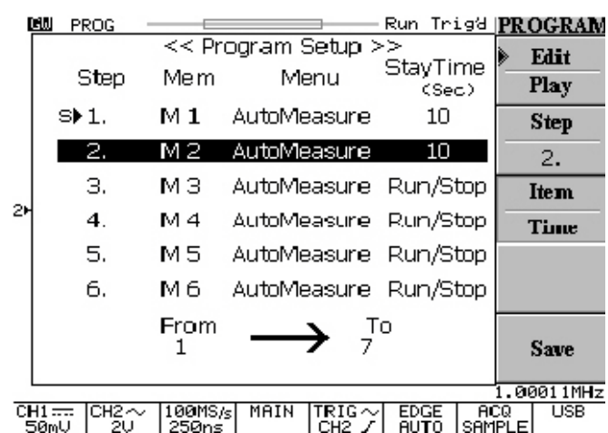
Figure 5-33: Editing the program condition of step two
