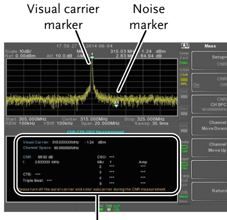
CNR measurements
