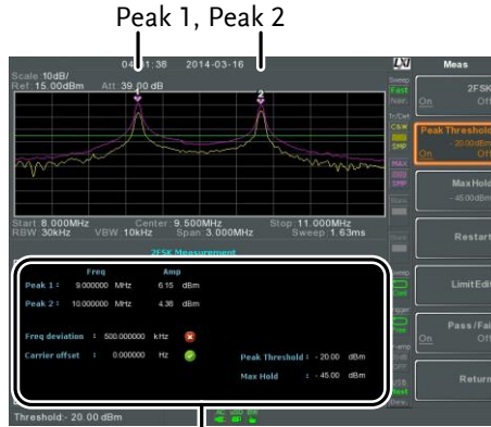
2FSK measurement
