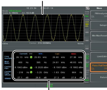
FM modulation measurements
