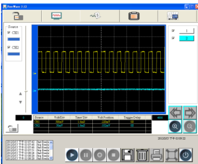
Two waveforms
