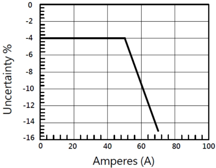
Figure 8. DC signal linearity in the 50 mV/A range, typical
