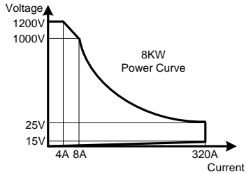
PEL-5008C-1200-320 power contour
