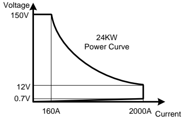
PEL-5024C-150-2000 power contour
