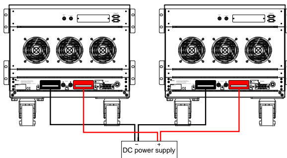
PEL-5000C series load parallel operation
