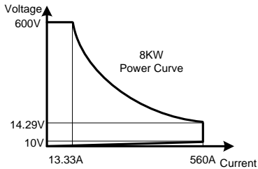
PEL-5008C-600-560 power contour
