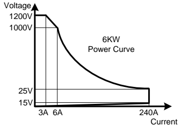
PEL-5006C-1200-240 power contour
