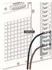
ASR-6000 AC One-phase Input
