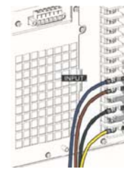
ASR-6000 AC Three-phase Input (Y Connection)
