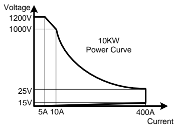
PEL-5010C-1200-400 power contour
